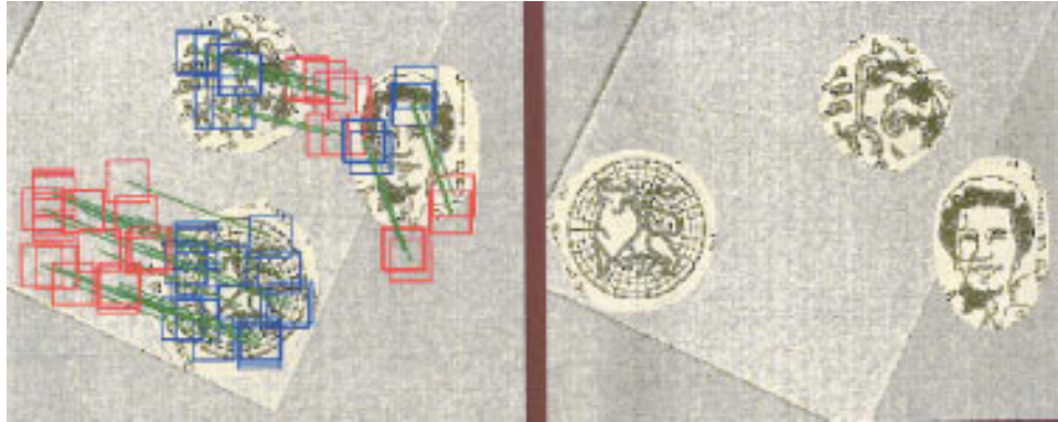
Figure 9.7: Results of applying Algorithm 3. At the right is the image at time t_1 . At the left is the image at time t_2 with the motion analysis overlaid. Red squares indicate the location of the original neighborhoods detected by the interest operator in the image at the right. Blue squares indicate the best matches to these neighborhoods in the image at the left. There are three coherent sets of motion vectors (green lines) corresponding to the three moving objects. Analysis courtesy of Adam Clark.
