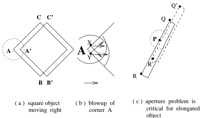
Figure 9.13: (a) A square object moves right; (b) a blowup of corner A shows how the constraints from two neighboring image flow equations can reduce the ambiguity of direction to \pi/2 . (c) An extreme aperture problem: an elongated object moves in the direction of its length; from the aperture around point P and its neighbors, the ambiguity in the direction of motion is \pi .
