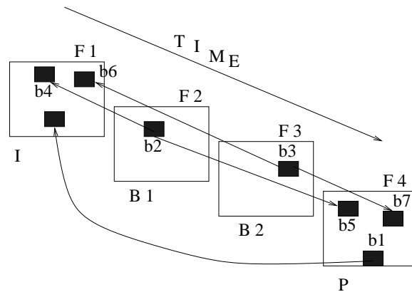
Figure 9.8: A coarse view of the MPEG use of motion vectors to compress the video sequence of four frames F1 , F2 , F3 , F4 . F1 is coded as an independent (I) frame using the JPEG scheme for single still images. F4 is a P frame predicted from F1 using motion vectors together with block differences: 16 x 16 pixel blocks ( b1 ) are located in frame F1 using a motion vector and a block of differences to be added. Between frames B1 and B2 are determined entirely by interpolation using motion vectors: 16 x 16 blocks ( b2 ) are reconstructed as an average of blocks ( b4 ) in frame F1 and ( b5 ) in frame F4. Between frames F2 and F3 can only be decoded after predicted frame F4 has been decoded even though these images were originally created before F4. Between frames yield the most compression since each 16 x 16 pixel block is represented by only two motion vectors. I frames yield the least compression.
