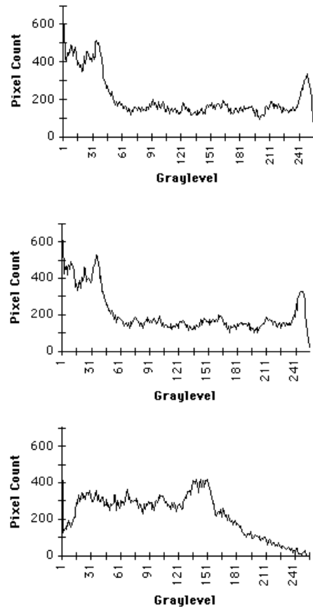
Figure 9.19: Histograms from the first three frames shown in Figure 9.18. The top two are similar as are the frames from which they were derived. The bottom histogram is significantly different from the top two, indicating that the frame from which it was derived is different from the first two. Reprinted from Zhang et al 1993 with permission from Springer-Verlag.
