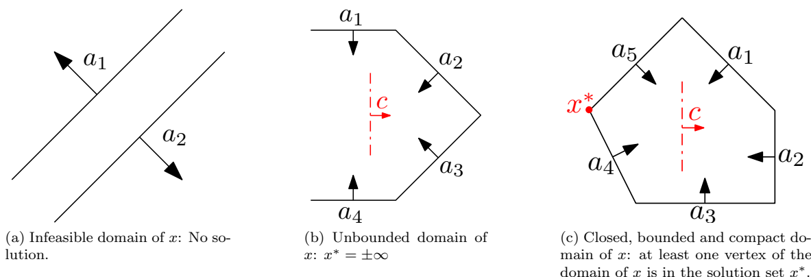
Figure 16.1: The possible domains of the solution variable x for an LP, along with the solution.
