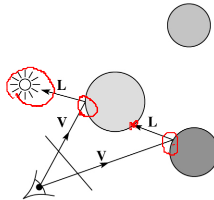
Shadow rays
