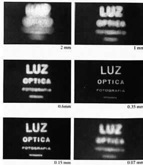
Diffraction
