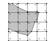
Isocontour from "marching squares"
