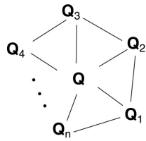
Vertex neighborhood
