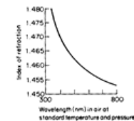
Index of refraction variation for fused quartz
