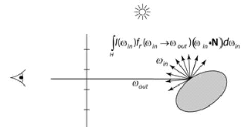
Reflection anti-aliasing
