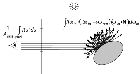
Pixel and reflection anti-aliasing
