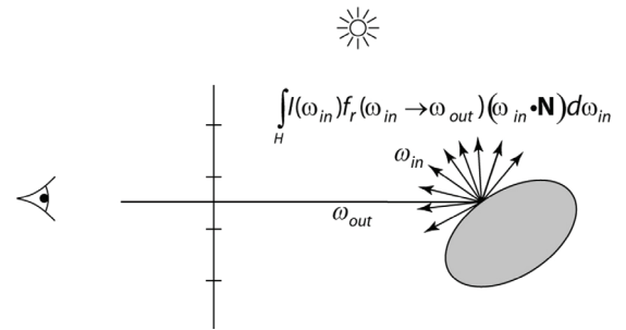
Reflection anti-aliasing
