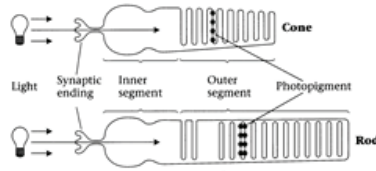
light gathering by rods and cones (Wandell, 3.2)
