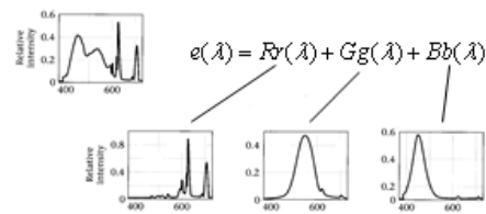
Emission spectra for RGB monitor phosphors (Wandell 2.3)
