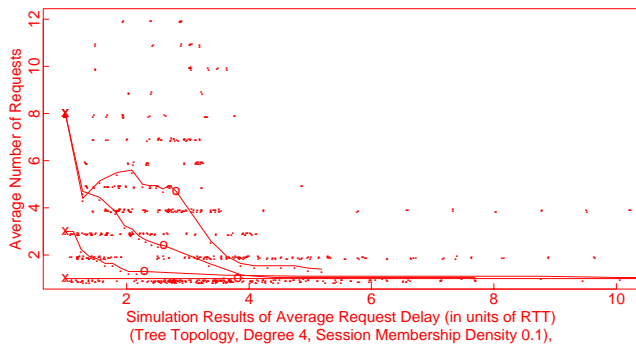
Figure 7: Tradeoff between delay and duplicates for dense sessions in tree topologies.
