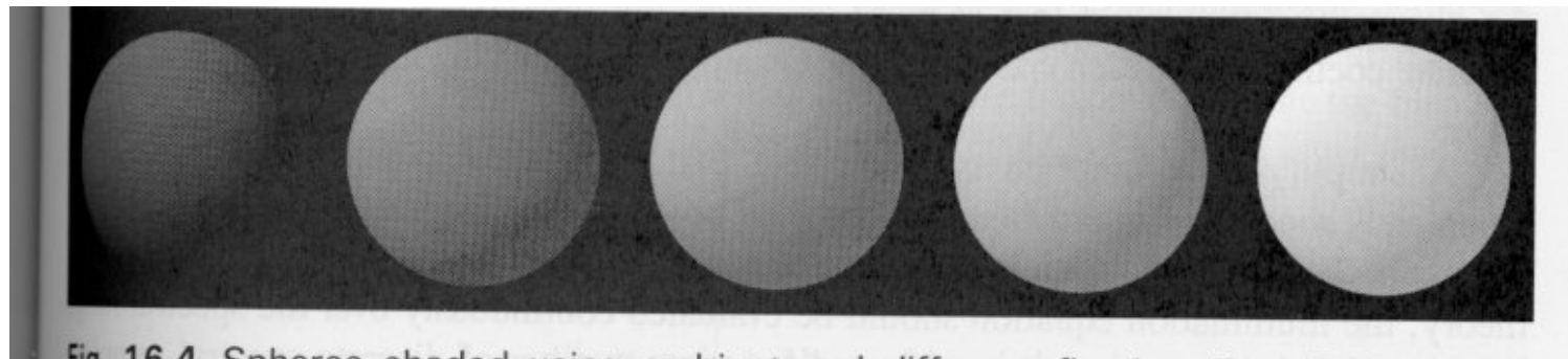
Fig. 16.4. Spheres shaded using ambient and diffuse reflection. From left to right, the ambient term increases from 0.0 to 1.0, and the diffuse term increases from 0.0 to 1.0.
