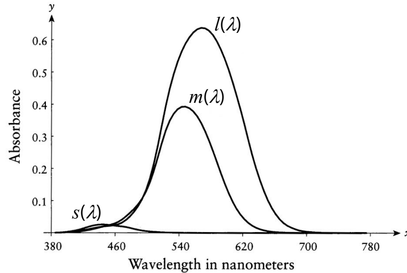
Cone photopigment absorption (Glassner, 1.1)
