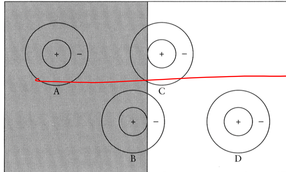
Lateral inhibition effect (Glassner, 1.25)
