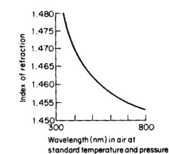
Index of refraction variation for fused quartz
