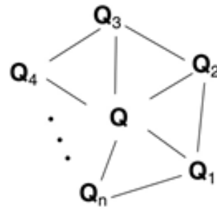
Vertex neighborhood
