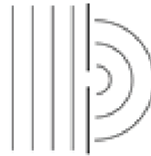
Diffraction
