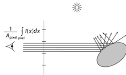
Pixel anti-aliasing
