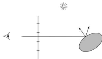
No anti-aliasing
