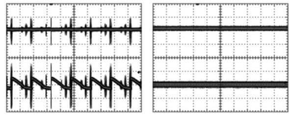
Figure 9: Version 1 (left) and Version 3 (right) Power supply noise. For each graph, the CPU power supply is shown on top (200mV/div), and the radio on the bottom (1V/div). The x-axis, time, is shown at 10µs/div.
