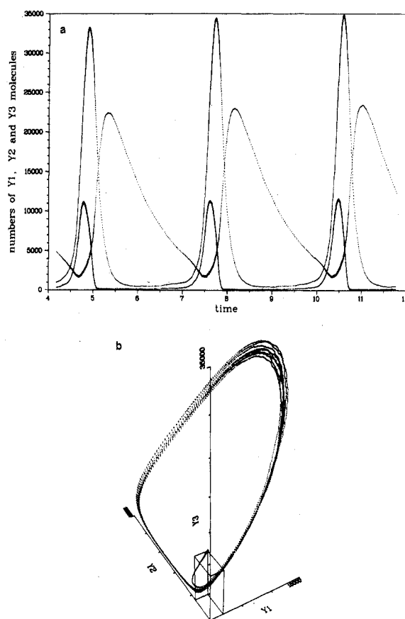
Figure 31. Showing the effects of increasing all molecular population levels in the Oregonator by a factor of 4 over their values in Figure 24: Y_{1_1} = 2000 , Y_{2_1} = 4000 , Y_{3_1} = 8000 , \rho_{1_1} = 2000 , and \rho_{2_1} = 50000 . (a) A 500 rpd plot of Y_1 (low-peaking curve), Y_2 (middle-peaking curve), and Y_3 (high-peaking curve) vs. t for 4 < t < 12 (cf. Figure 24b). (b) A 1000 rpd plot of the trajectory in Y_1Y_2Y_3 space for 0 \leq t \leq 24 (cf. Figure 24c).
