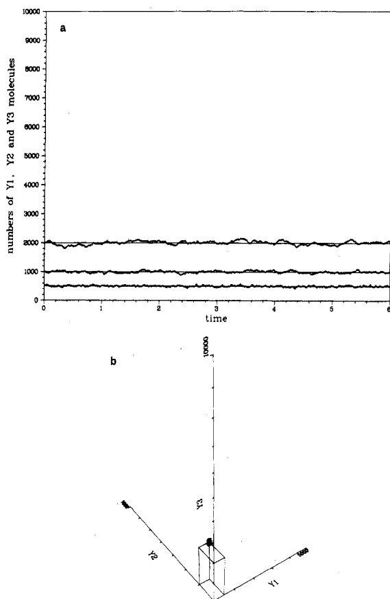
Figure 30. Same as Figures 24a and 24c, except that \rho_{1_1} = 5000 and \rho_{2_1} = 5000 .
