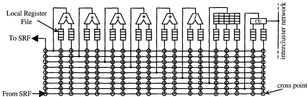
Figure 5: Imagine Cluster Organization
