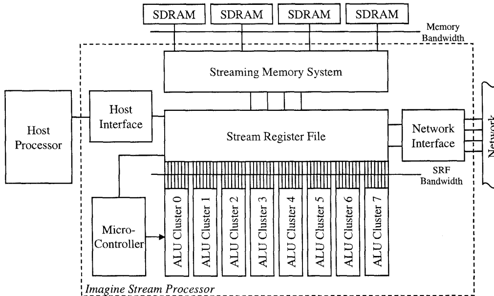
Figure 3: Block Diagram of Imagine
