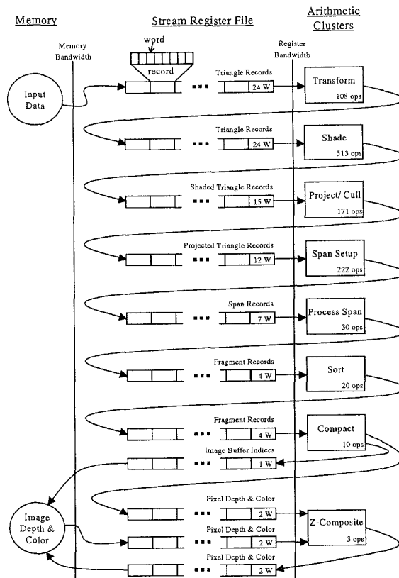
Figure 1: Stream-Based Triangle Rendering
