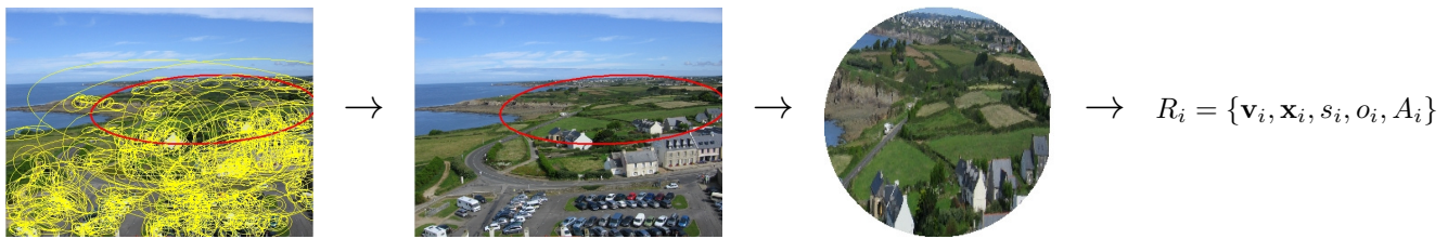
Figure 2. Image analysis stage, as done by a typical local description program. Regions of interest are first detected and affine-normalized to a fixed-size square patch, which is subsequently described by a local descriptor and additional meta-data used in geometrical verification. Note that in our reconstruction approach (see Section 3), we will reconstruct elliptic patches out of normalized circular patches.
