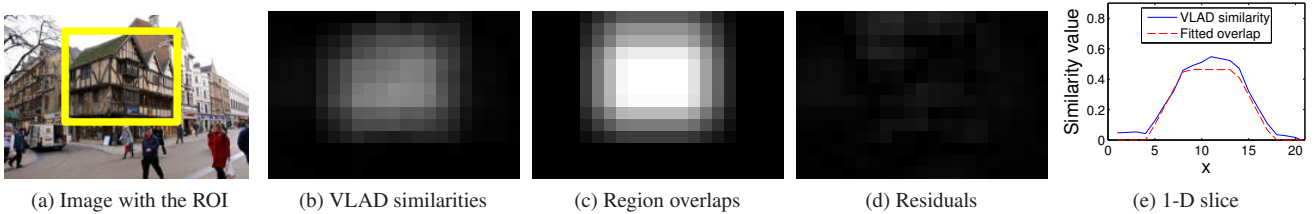
Figure 4: Variation of VLAD similarity with region overlaps. (b) The value plotted at each point (x, y) corresponds to the VLAD similarity (scalar product between two VLADs) between the VLAD of the region of interest (ROI) in (a) and the VLAD extracted from the 200 \times 200 pixel patch centered at (x, y) . (c) The proportion of each patch from (b) that is covered by the ROI from (a). (d) Residuals obtained by a linear regression of (c) to (b). (e) A 1-D horizontal slice through the middle of (b) and (c). Note that residuals in (d) and (e) are very small, thus VLAD similarities are very good linear estimators of region overlap.
