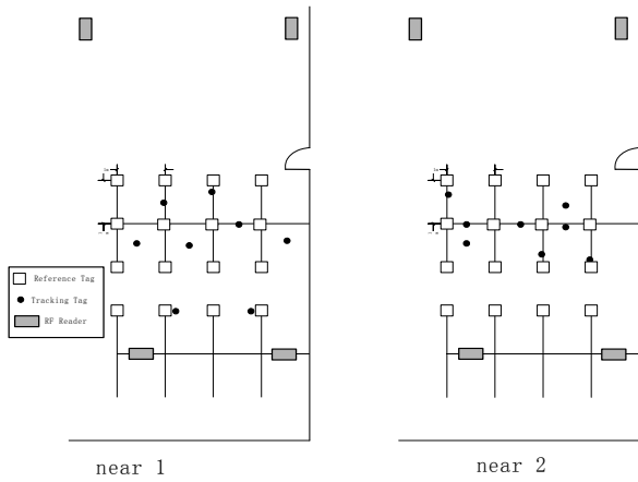
Figure 11: Two higher density, comparing with those in Fig. 4, placements of reference tags
