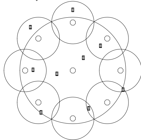
Figure 3: Placement of 9 readers with two different ranges and the sub-regions.
