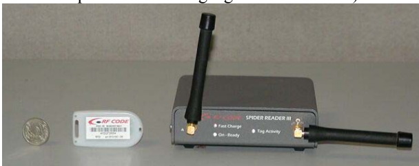
Figure 2: The RFID reader and tag used in our prototype system.
