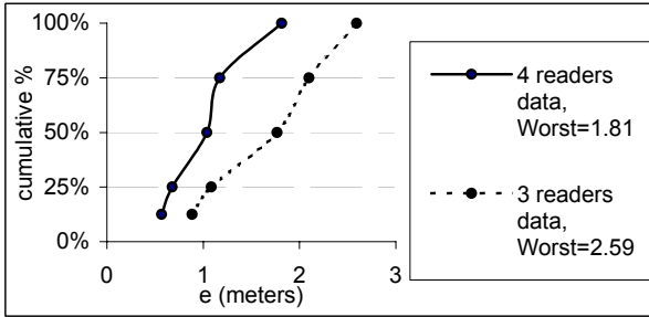
Figure 8: Cumulative percentile of error distance for 3 and 4 RF readers.
