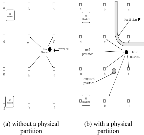
Figure 9: A physical partition to separate reference tags c and f from others
