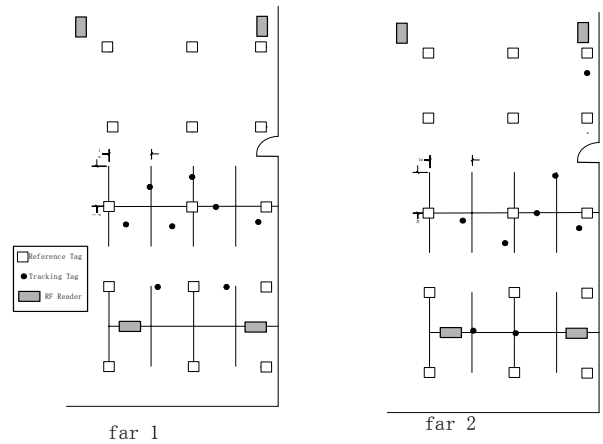
Figure 13: Two lower density, comparing with those in Fig. 4, placements of reference tags
