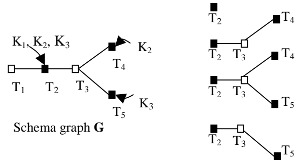
Figure 4. Join trees
