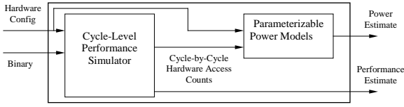
Figure 2: Overall Structure of the Power Simulator.
