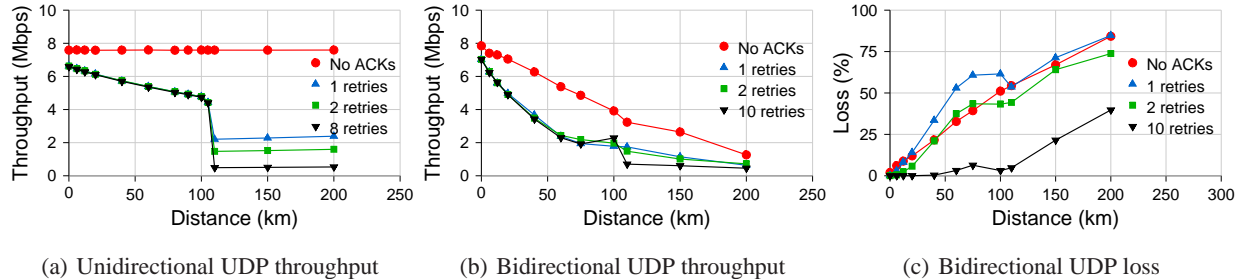
Figure 2: UDP throughputs for standard 802.11 CSMA on single emulated link. ACK timeouts were adjusted with increasing distance (on Atheros cards). Traffic is 1440 byte CBR UDP packets in 802.11b at PHY layer datarate of 11Mbps.
