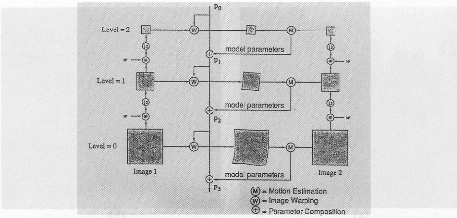
Fig. 1. Diagram of the hierarchical motion estimation framework.
