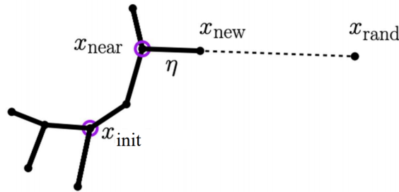
Figure 1: Visualization of extend() with step size \eta , which controls the ratio of the distance from x_{\text{near}} (the state to be extended) to x_{\text{new}} and the distance from x_{\text{rand}} (a sampled state) to x_{\text{near}} . If it is set to one, x_{\text{new}} = x_{\text{rand}} .
