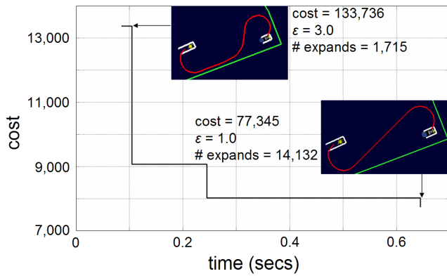
(a) anytime behavior
