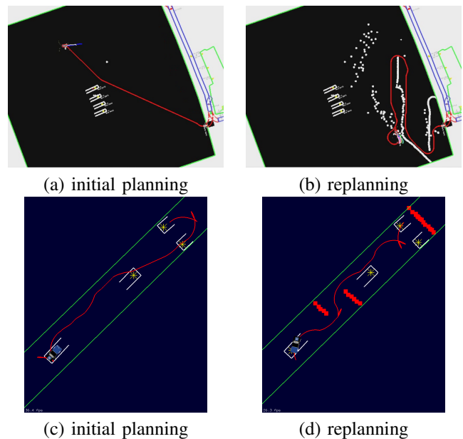
Fig. 9. Planning and replanning in large (a,b) and highly-constrained (c,d) environments
