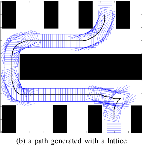
Fig. 1. (a) shows a 3D (x, y, \theta) lattice with at most five forward actions for each state and no backward actions. A full set of actions is shown for state s_1 . For every state, this set of actions is translated and rotated appropriately, and all actions intersecting obstacles are removed. (b) shows an example of a complex 3D path for a vehicle with a large rectangular footprint (obstacles are shown in black).
