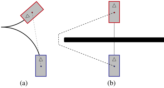
Fig. 4. Mechanism-constrained (solid) and environment-constrained (dashed) heuristic paths. In each case, the initial and desired vehicle poses are shown as blue and red rectangles, respectively (with the interior triangles specifying the headings). (a) The mechanism-constrained heuristic is perfectly informed when no obstacles are present in the environment. (b) The environment-constrained 2D heuristic can provide significant benefit when obstacles exist. Here, an obstacle (shown in black) resides over the direct path to the desired pose.
