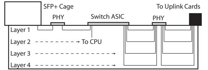
Fig. 6: Layers of the pod switch line card circuit board. This figure is not to scale.
