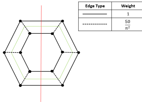
Figure 14.1: A weighted graph comprised of two cycles. The conductance of the red cut is n times the conductance of the green cut, but the spectral partitioning algorithm returns the red cut.
