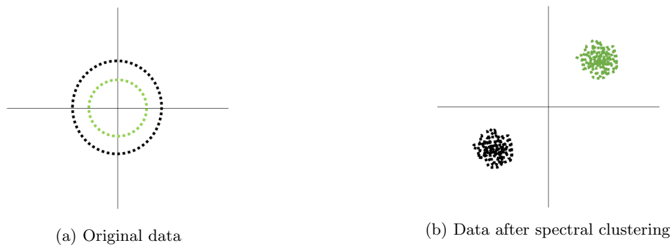
Figure 14.2: Spectral clustering: before and after
