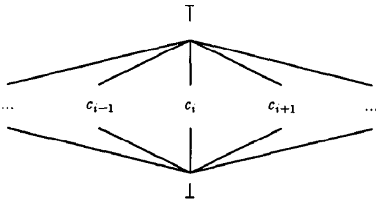
Figure 3. The constant propagation lattice.
