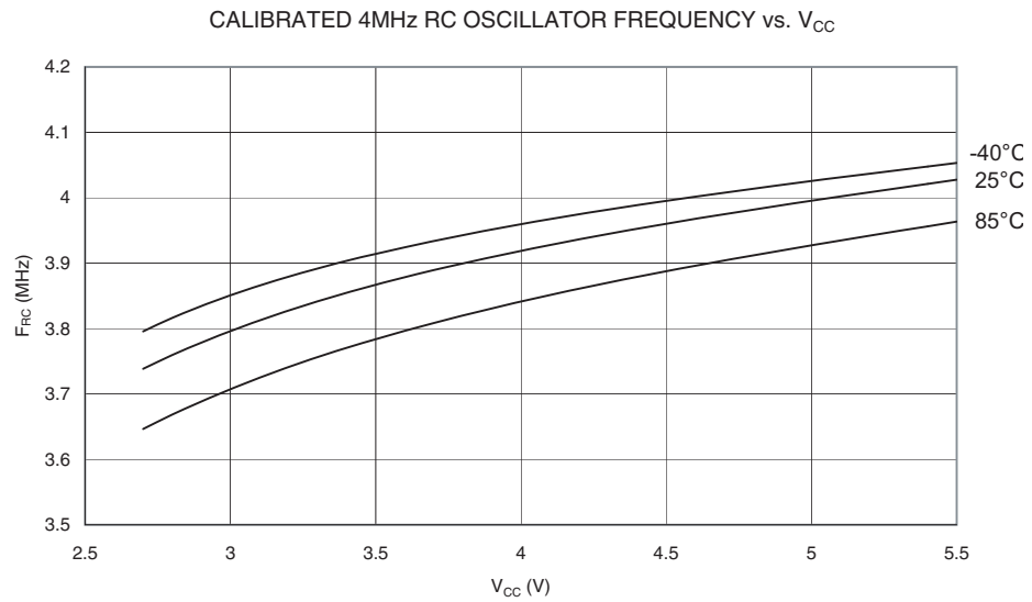
Figure 198. Calibrated 4 MHz RC Oscillator Frequency vs. V_{CC}
