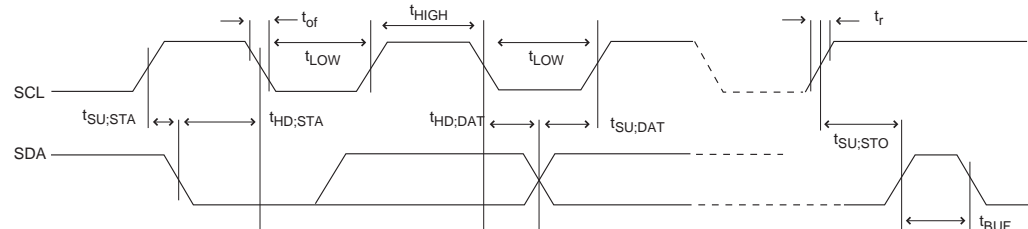
Figure 146. Two-wire Serial Bus Timing
