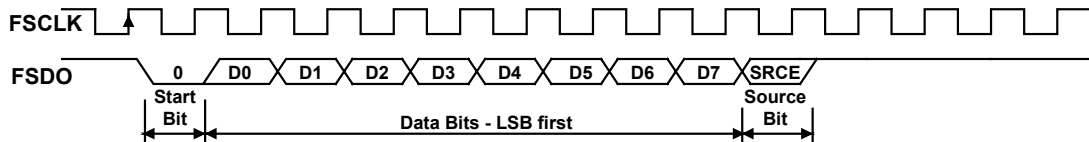
Figure 34 - Fast Opto-Isolated Serial Data Format - Data output from the FT2232C
