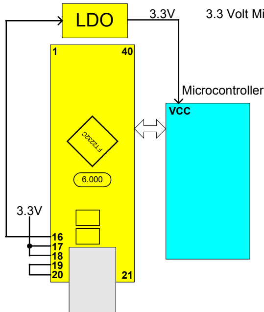
Figure 10c - Bus Powered
