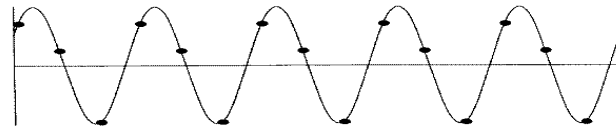
Figure 3.15 When a sine wave is sampled three times per cycle ( f_s = 3f ), the observed frequency is equal to the true frequency.
