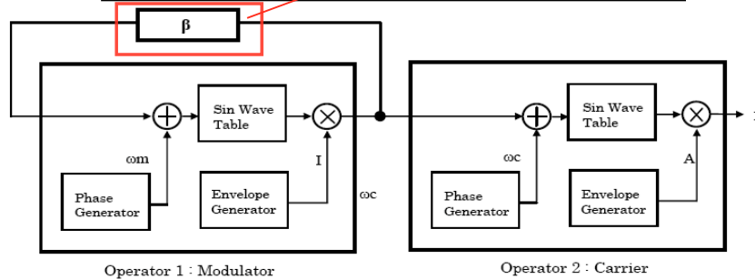
Operator 1 : Modulator
