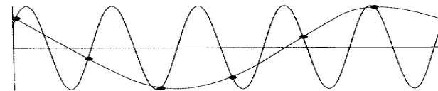
Figure 3.16 When a sine wave is sampled six times in five cycles, the observed sine wave has a much lower frequency than the original sine wave.
