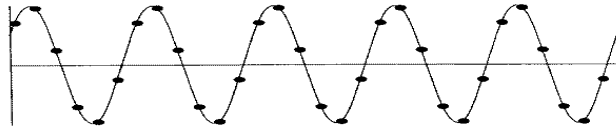
Figure 3.14 When a sine wave is sampled six times per cycle ( f_s = 6f ), the observed frequency is equal to the true frequency.
