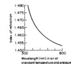
Index of refraction variation for fused quartz
