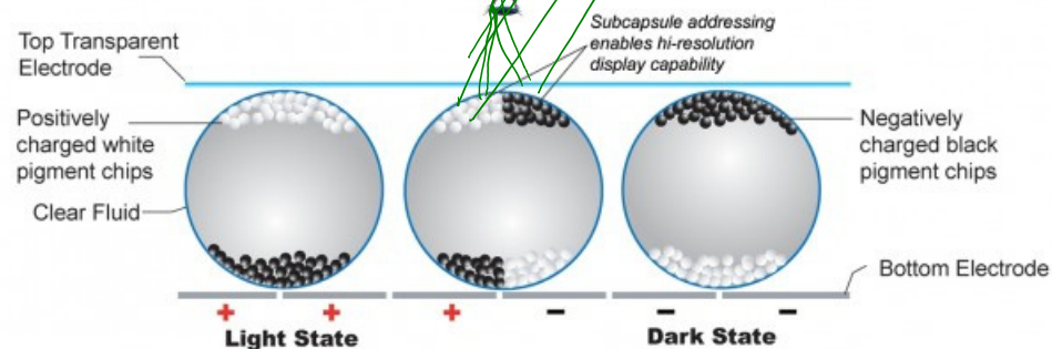
Cross-Section of Electronic-Ink Microcapsules
