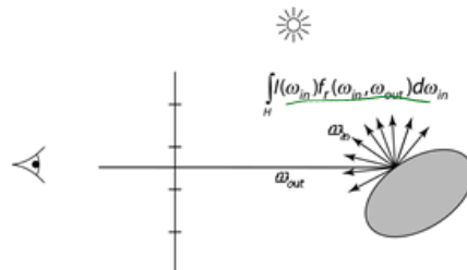
Reflection anti-aliasing
