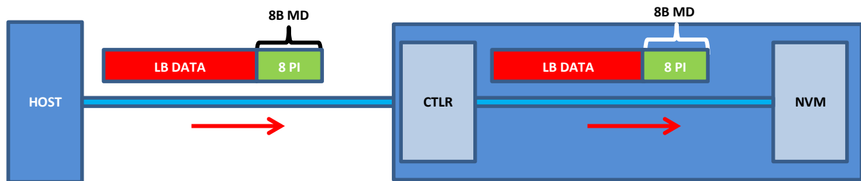
Figure 216: Write Command Protection Information Processing
