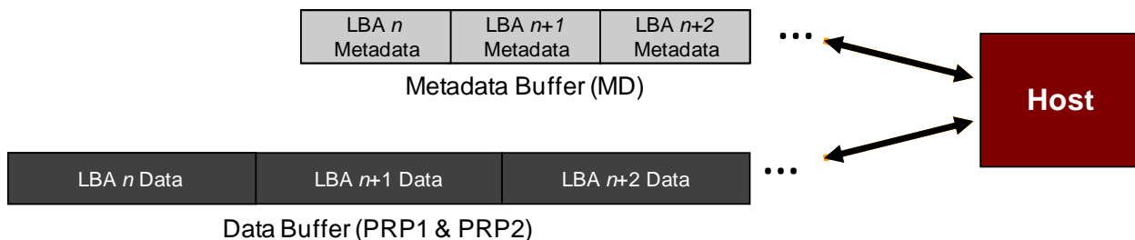
Figure 214: Metadata – Transferred as Separate Buffer
