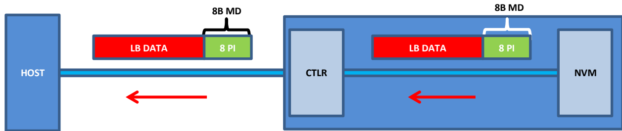
Figure 217: Read Command Protection Information Processing
