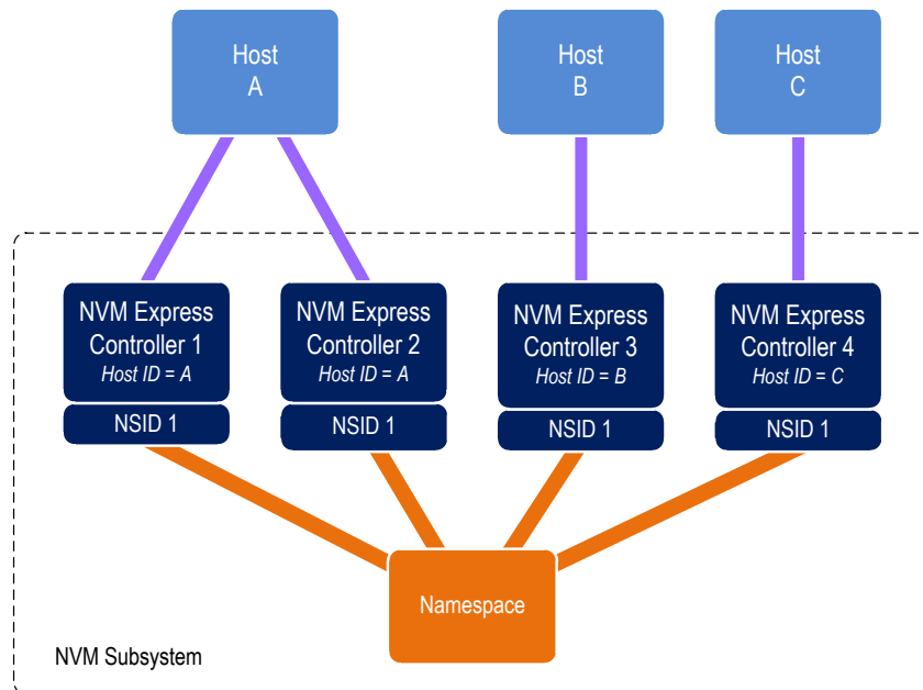
Figure 222: Example Multi-Host System
