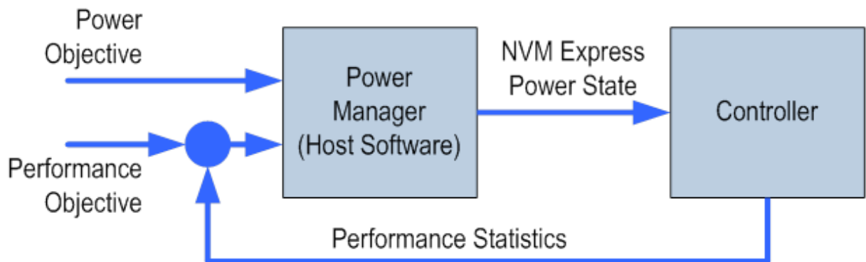
Figure 219: Dynamic Power Management
