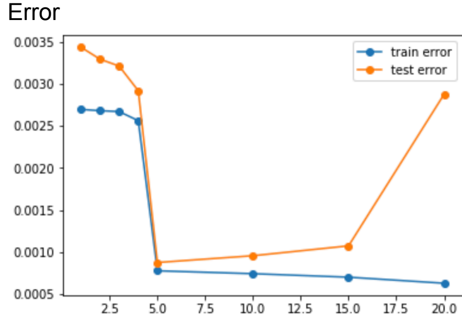
Degree- p polynomial model
