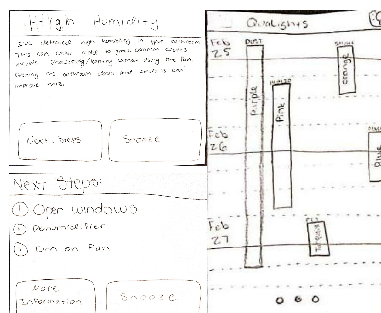
Paper Prototyping
