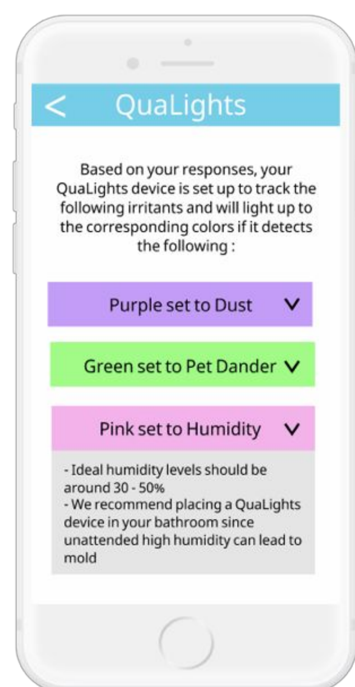
Personalize Notifications
