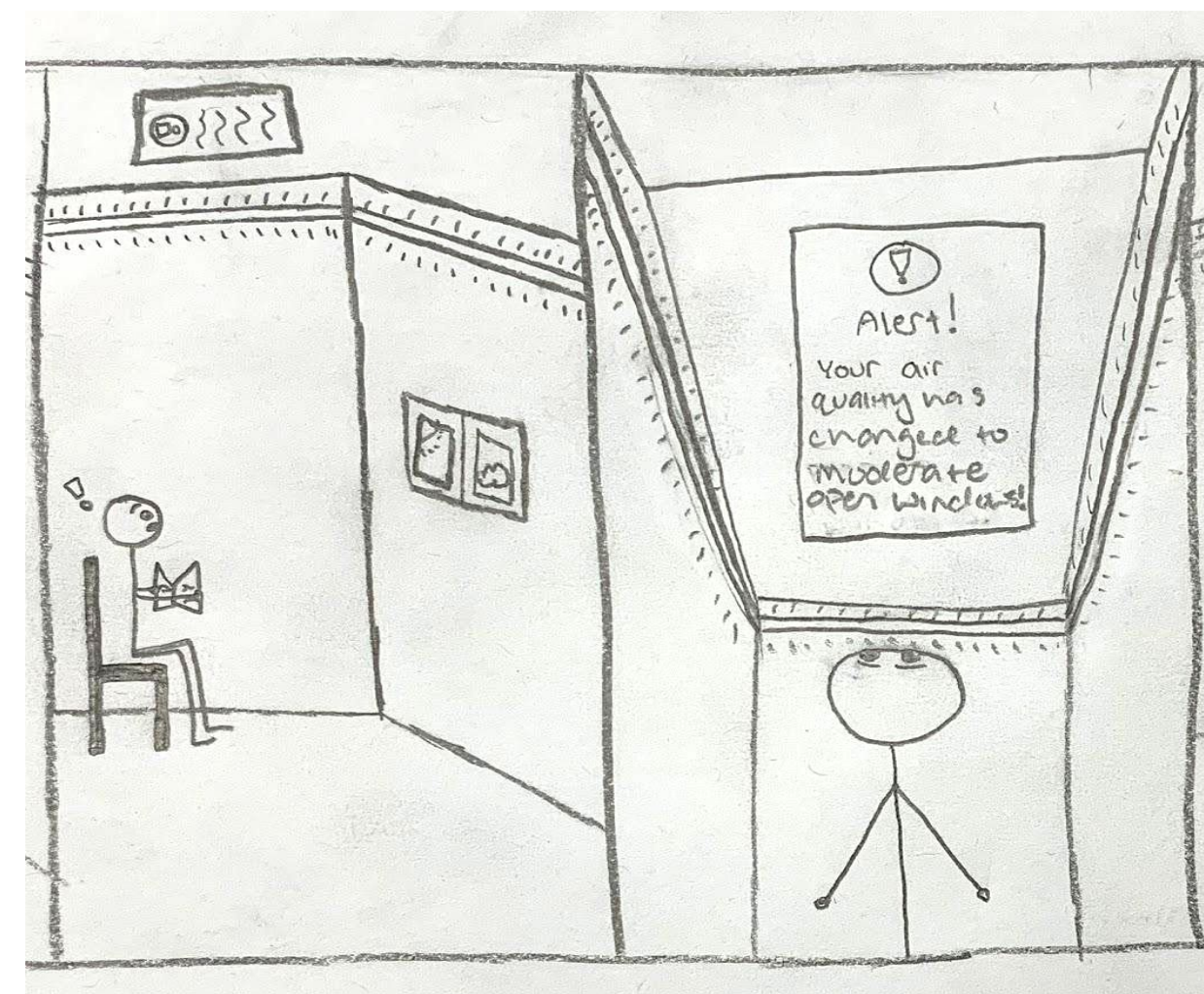
Storyboarding
