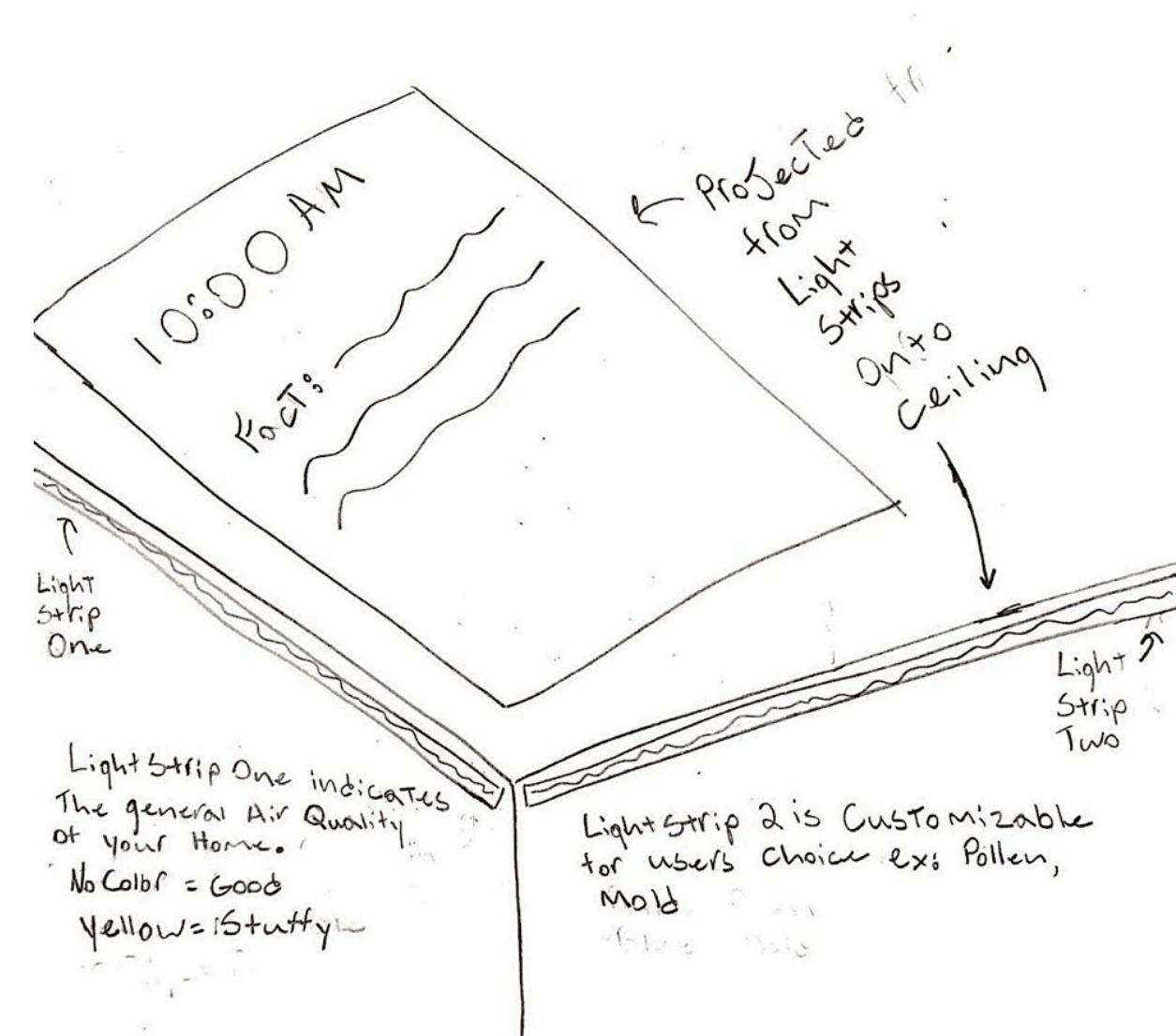
Sketching
