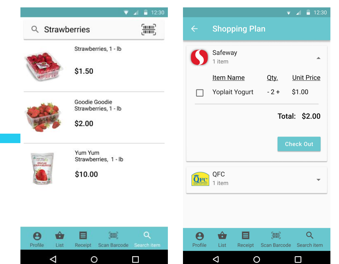
Digital Mockup
