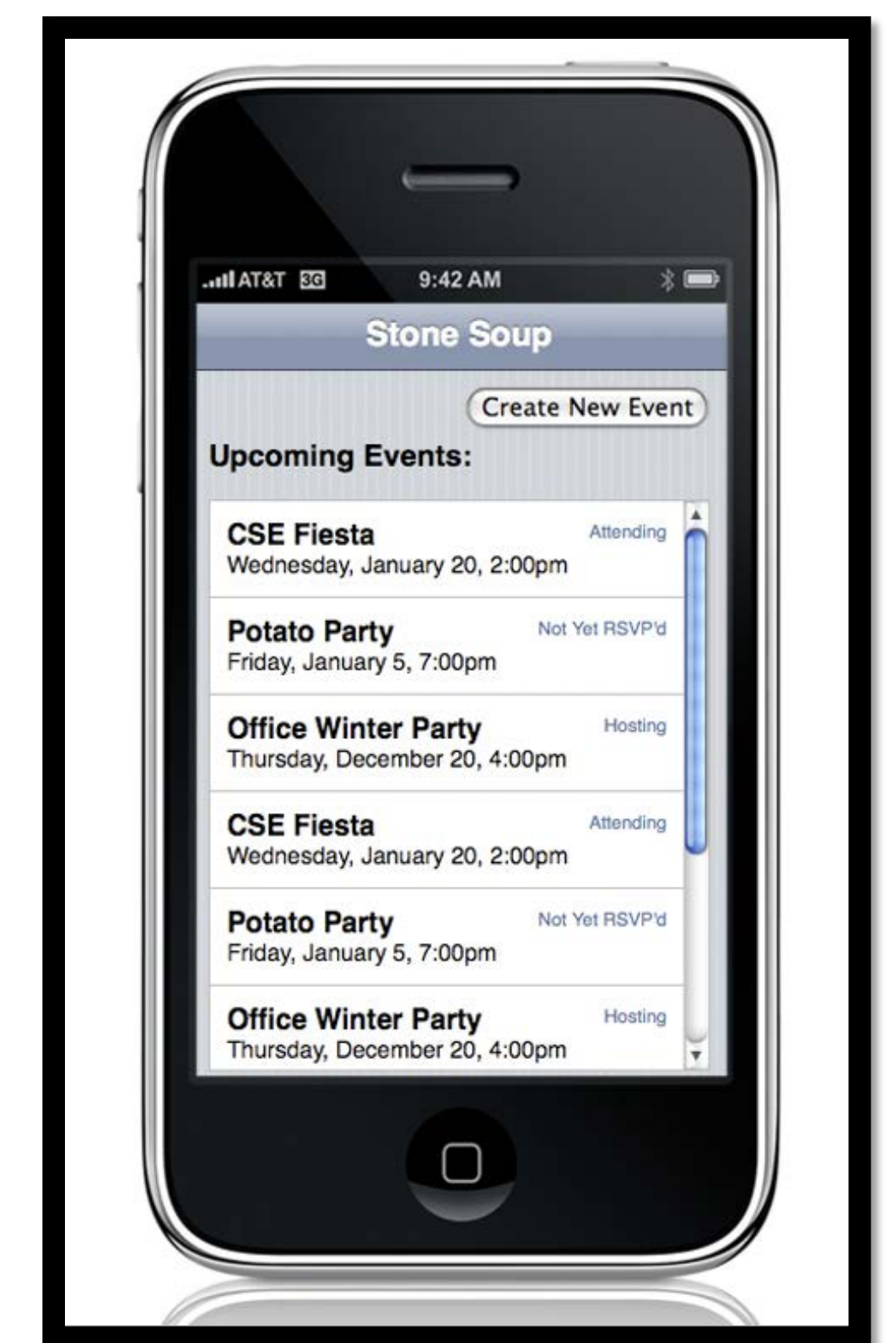
Interactive Prototype
