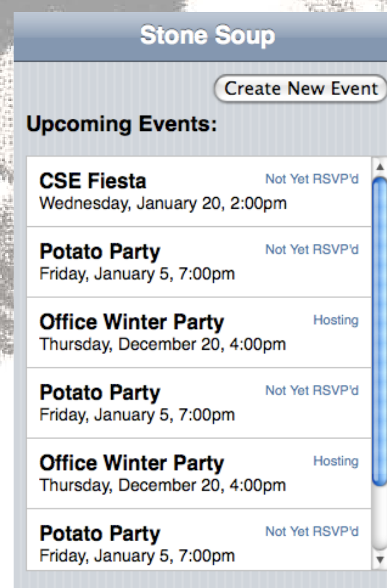
Home Screen
