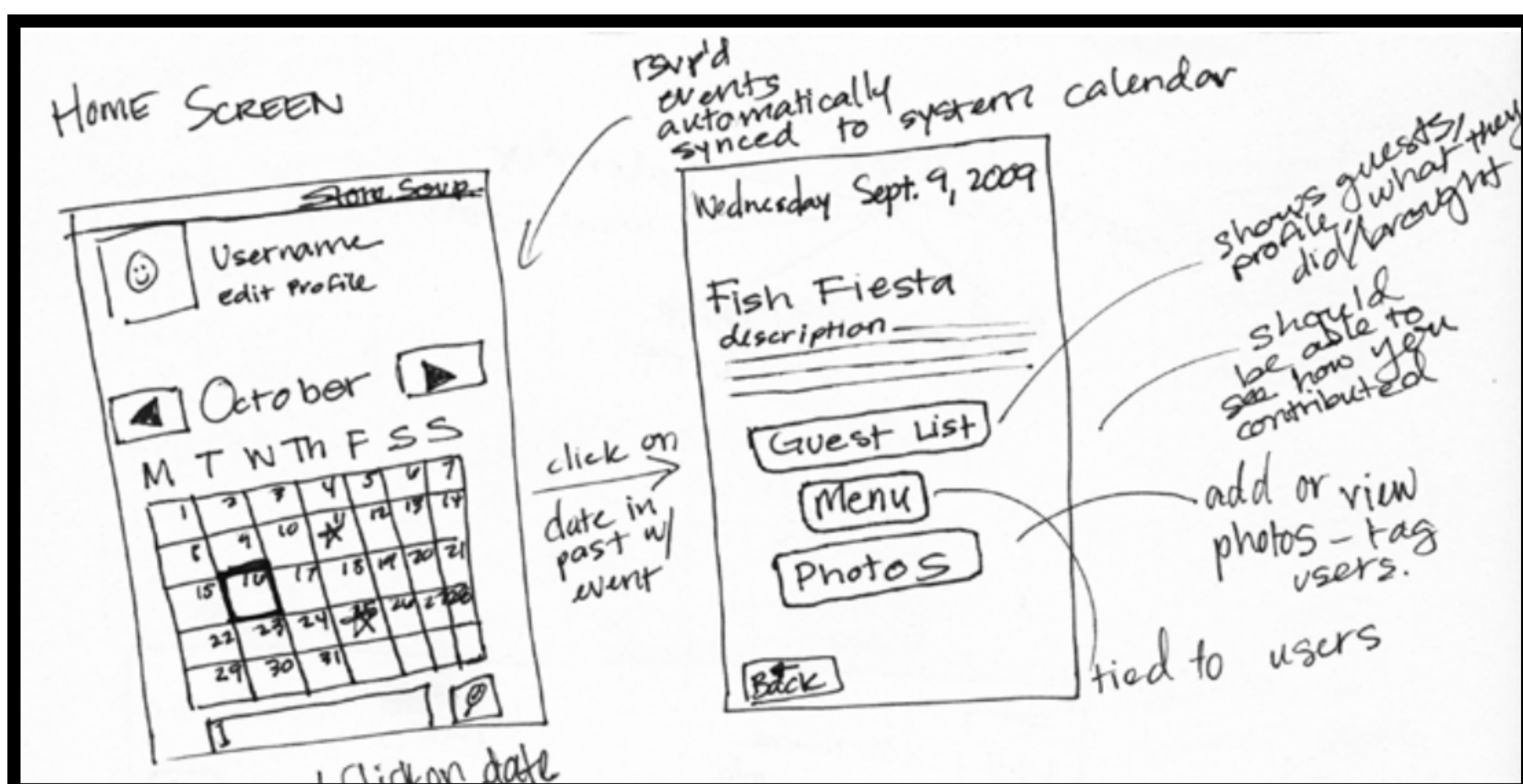
Early Sketches
