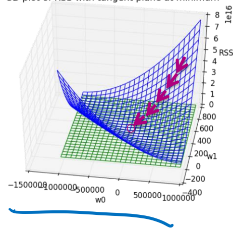
3D plot of RSS with tangent plane at minimum
