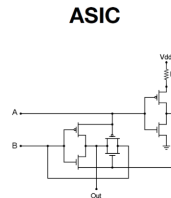
just 6 transistors
