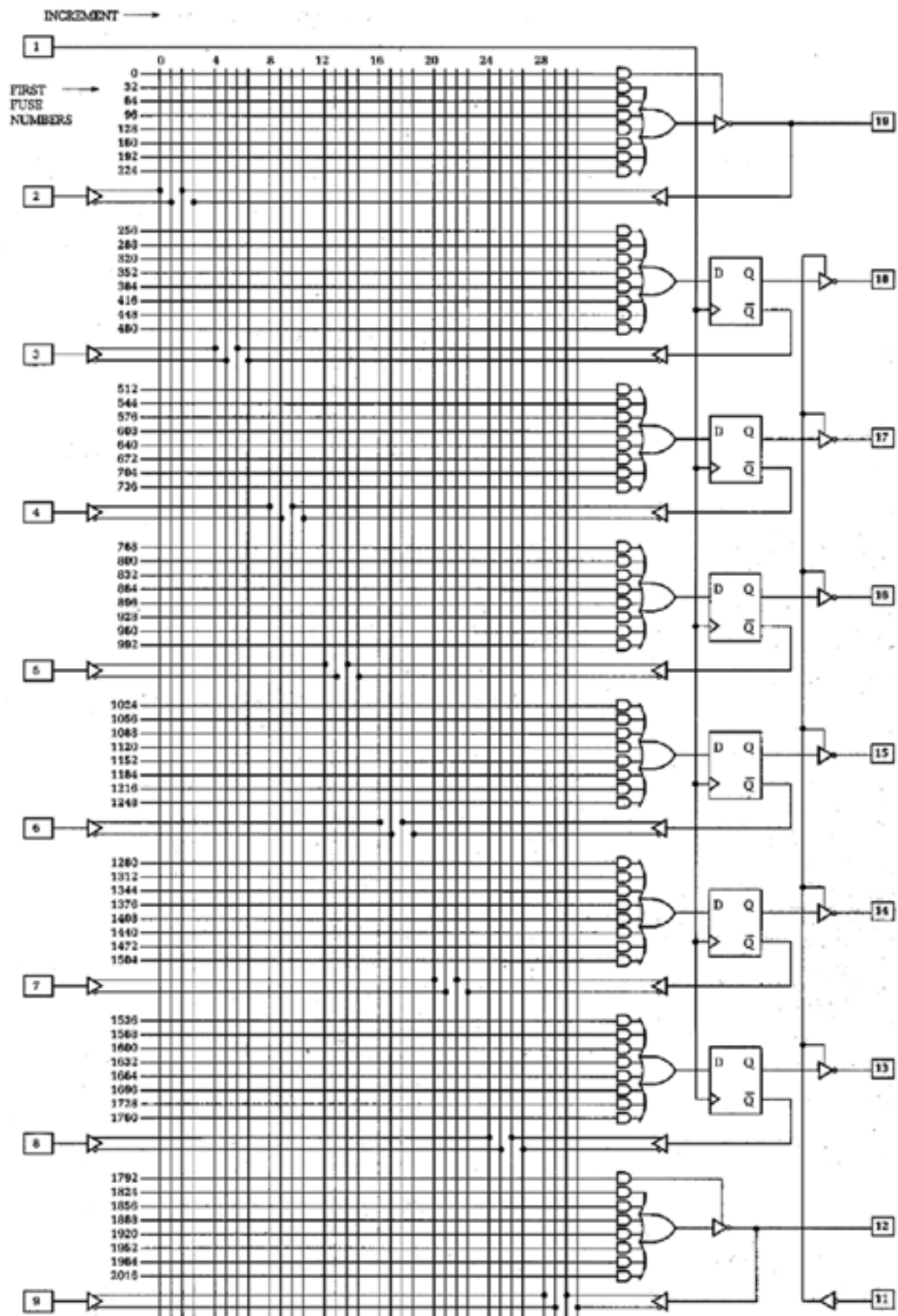
Figure 10.18 Registered 16R6 PAL.
