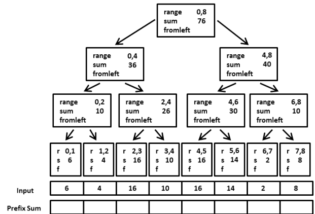
Figure 9: Example of the first pass of the parallel prefix-sum algorithm: the overall result (bottom-right) is a binary tree where each node holds the sum of a range of elements of the input. Each node holds the index range for which it holds the sum (two numbers for the two endpoints) and the sum of that range. At the lowest level, we write r for range and s for sum just for formatting purposes. The fromleft field is used in the second pass. We can build this tree bottom-up with \Theta(n) work and \Theta(\log n) span because a node's sum is just the sum of its children.
