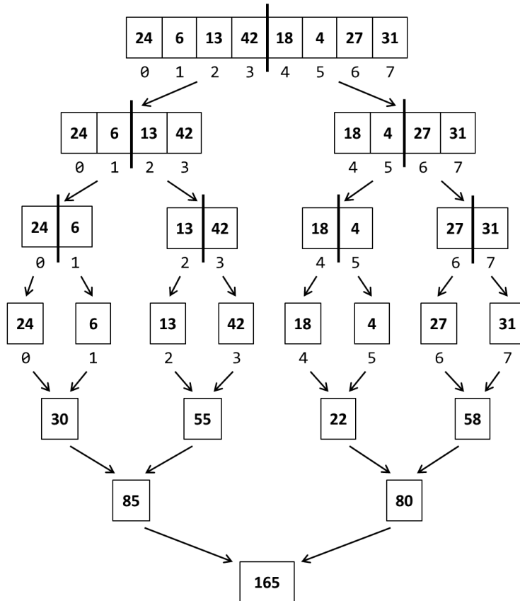
Figure 7: Example execution dag for summing an array.
