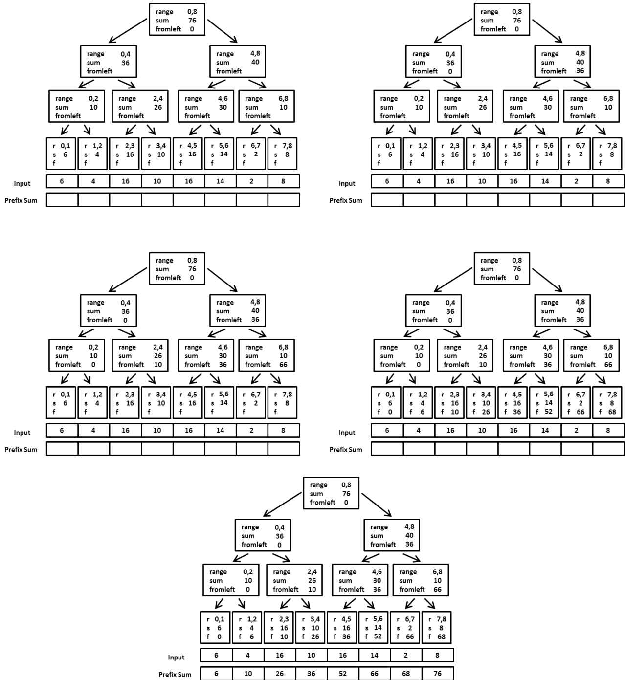
Figure 10: Example of the second pass of the parallel prefix-sum algorithm. Starting with the result of the first pass and a “fromleft” value at the root of 0, we proceed down the tree filling in fromleft fields in parallel, propagating the same fromleft value to the left-child and the fromleft value plus the left-child’s sum to the right-value. At the leaves, the fromleft value plus the (1-element) sum is precisely the correct prefix-sum value. This pass is \Theta(n) work and \Theta(\log n) span.
