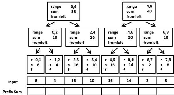
Figure 9: Example of the first pass of the parallel prefix-sum algorithm: the overall result (bottom-right) is a binary tree where each node holds the sum of a range of elements of the input. Each node holds the index range for which it holds the sum (two numbers for the two endpoints) and the sum of that range. At the lowest level, we write r for range and s for sum just for formatting purposes. The fromleft field is used in the second pass. We can build this tree bottom-up with \Theta(n) work and \Theta(\log n) span because a node's sum is just the sum of its children.
