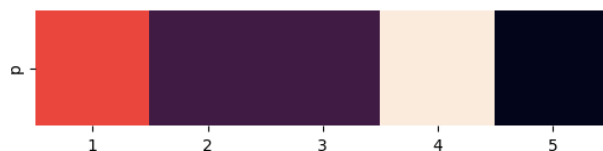
Figure 9.6.3: Belief Distribution vP^5 at n = 5
