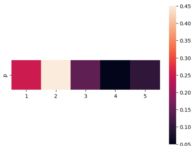
Figure 9.6.1: Belief Distribution v at n = 0
