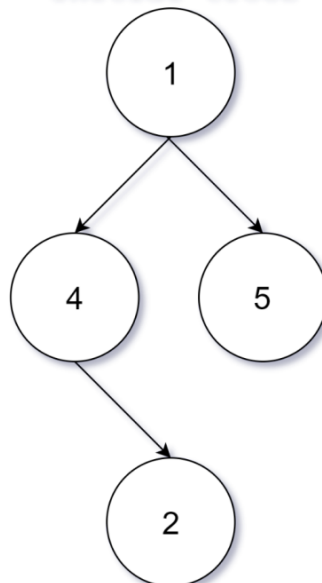
initial tree2
