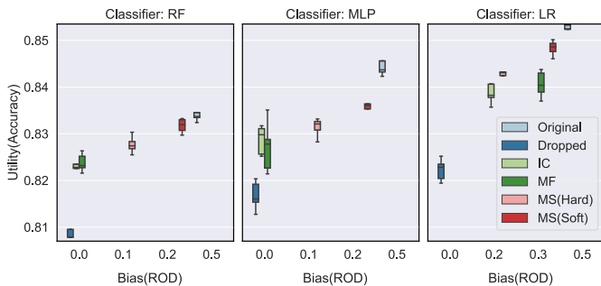
Figure 7: Performance of CAPUCHIN on Adult data.
