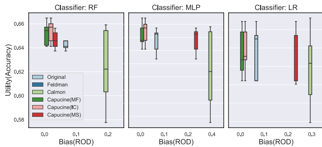
Figure 14: Comparison with other methods on Binned COMPAS.
