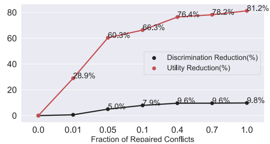
Figure 11: Bias-utility trade off in MaxSAT approach.
