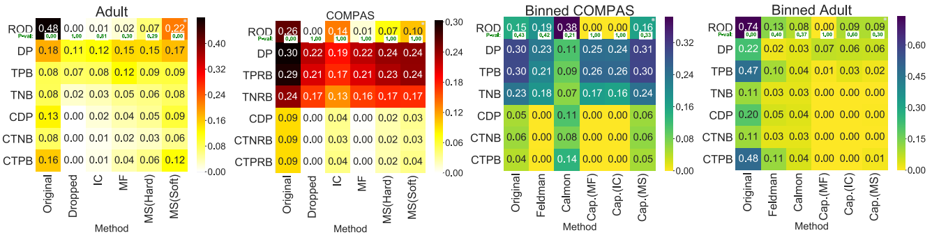
Figure 8: Bias reduction performance of CAPUCHIN for MLP classifier.
